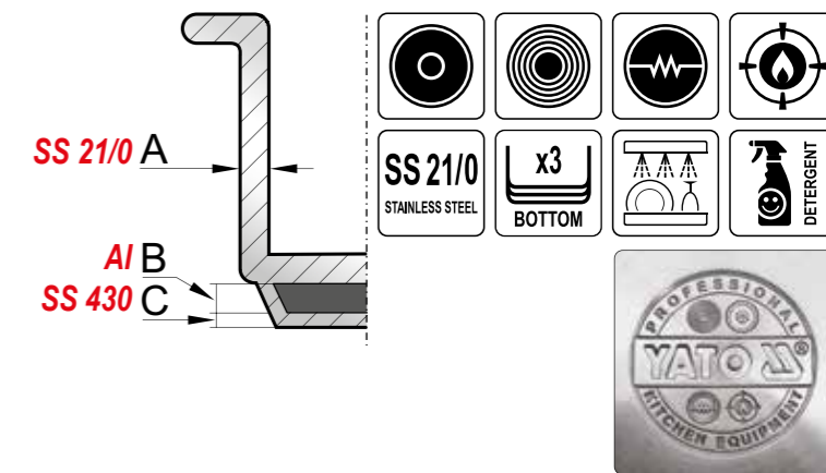
Distribution of heat throughout the bottom
